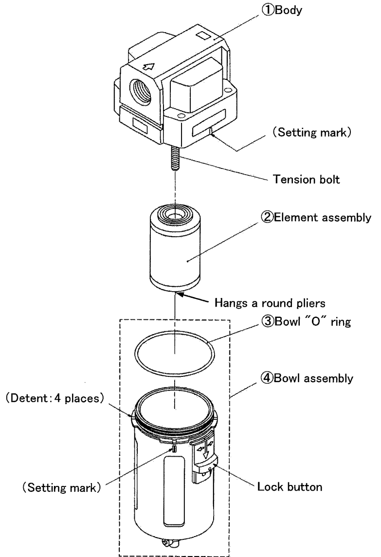
2)AFM30/40 Disassembly drawing
