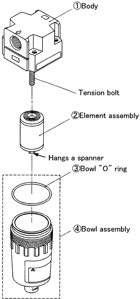
1)AFM20 Disassembly drawing
