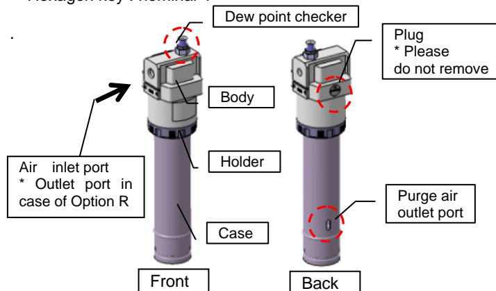
Fig 2.1 Names of parts (Example: IDG30□A)
