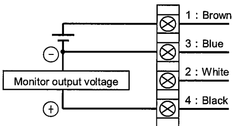
Analogue output - Voltage type (ITVX2030-※1)
