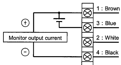
Analogue output - Current (sink) type (ITVX2030-※4)
