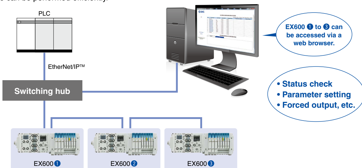
Connection example
