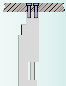
③ Vertical mounting (Body tapped)
