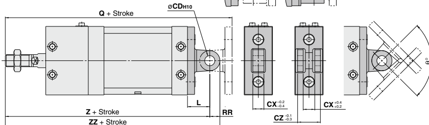
Single clevis type Double clevis type
