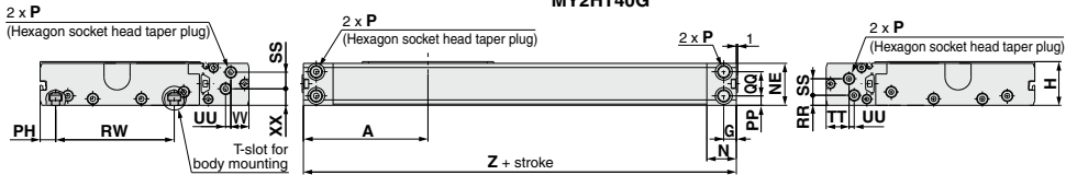
T-slot for body mounting
