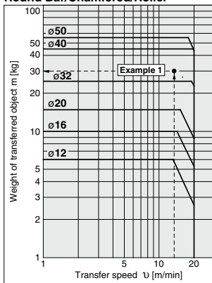
Graph 1 Round Bar/Chamfered/Roller
