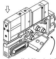
Hook this part onto the DIN rail, and press down in the direction of the arrow.
