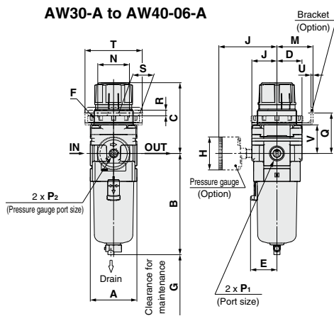
Panel fitting dimensions
