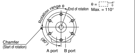
The above figure shows the CRB2 series. (Viewed from the long shaft side)
