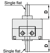
Double shaft/CRB2□Y
