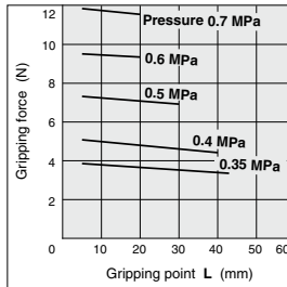
MHZ2-16S/MHZL2-16S
