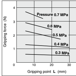
MHZ2-10S/MHZL2-10S
