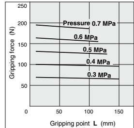
MHZ2-40S
