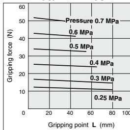
MHZ2-20S/MHZL2-20S
