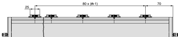
Emitter cartridge
