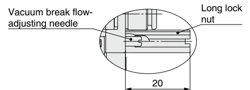
H (2 : 1) ZK2□□A5MOZ□□-□□-□□E-X188
